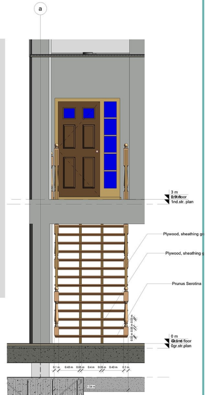
2 Grand floor stair details 2 1 : 20
