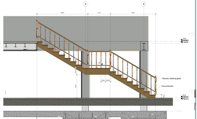
1 grand floor stair details 1 1 : 20
